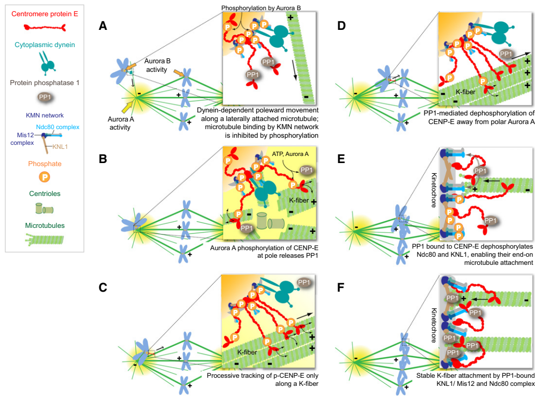
Figure 7. A Model of CENP-E Regulation by Aurora Kinases and PP1
