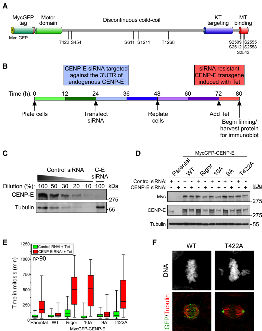
Figure 3. Phosphorylation of CENP-E at T422 Is Required for Chromosome Alignment
