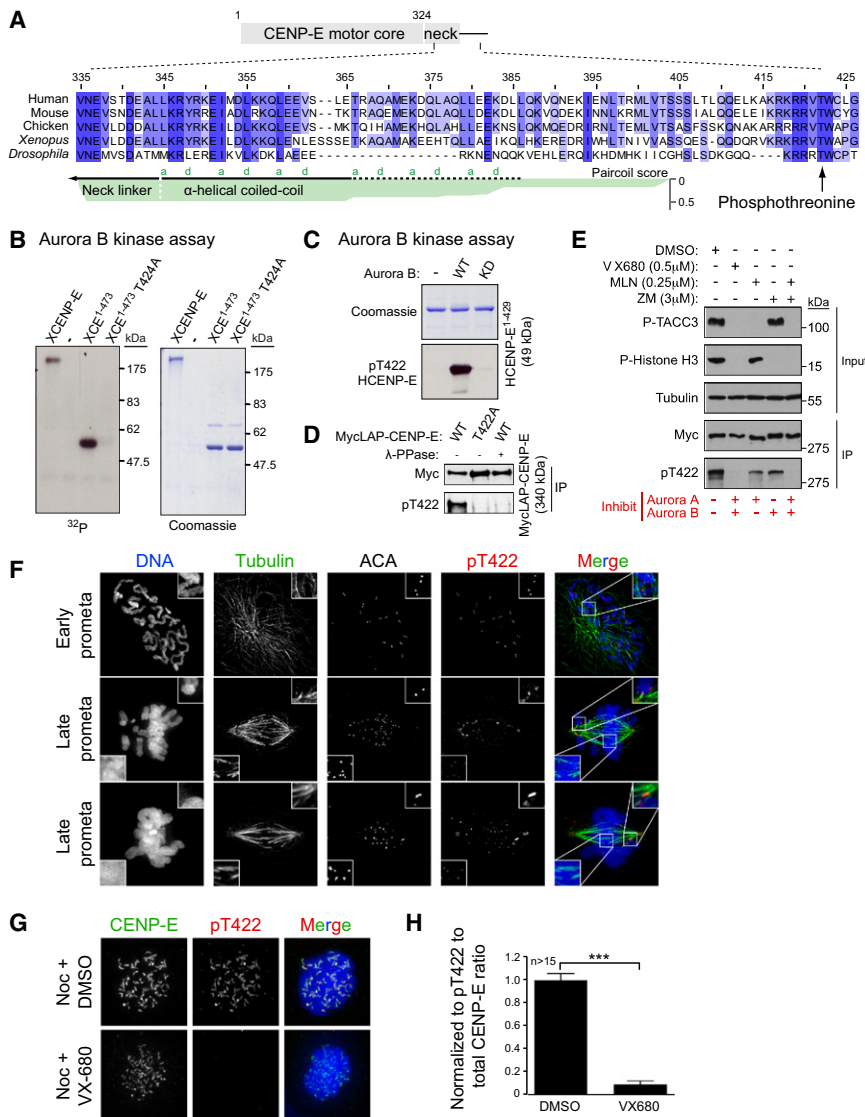
Figure 1. A Conserved Threonine Close to the Motor Domain of CENP-E Is Phosphorylated by Aurora A and B on the Kinetochores of Unaligned Chromosomes
