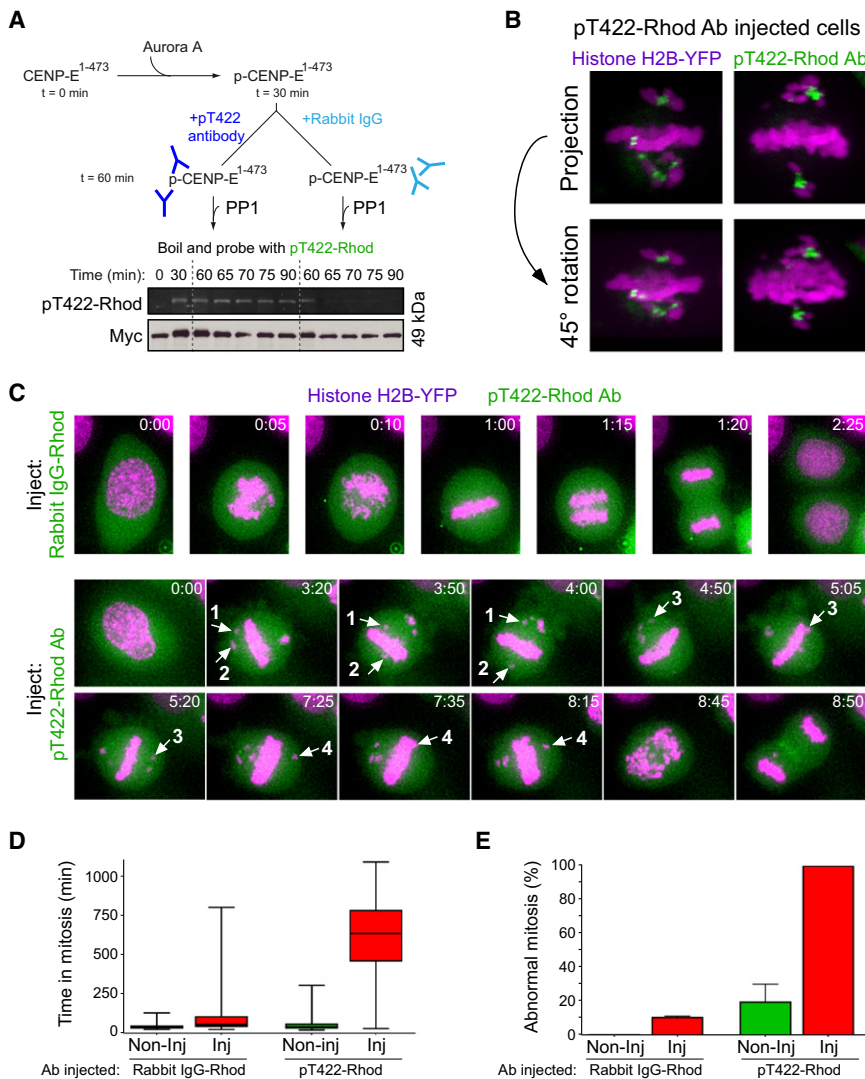
Figure 6. Dephosphorylation of CENP-E T422 by PP1 Is Required for the Stable Bio-orientation of Chromosomes Congressed from a Spindle Pole by CENP-E
