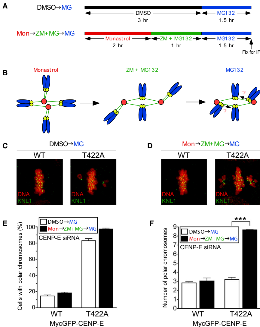
Figure 4. CENP-E Phosphorylation by Aurora Is Required for Congression of Polar Chromosomes
