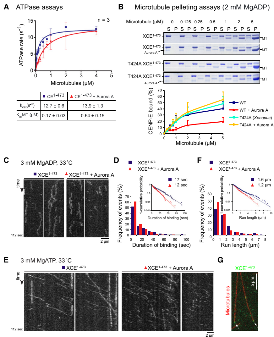
Figure 2. Phosphorylation of T424 of Xenopus CENP-E by Aurora Kinase Reduces CENP-E's Affinity for Microtubules and Reduces Its Run Length In Vitro
