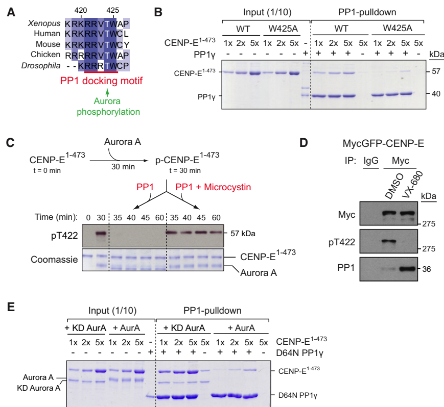
Figure 5. Aurora Phosphorylation of CENP-E T422 Opposes Direct Binding of CENP-E to PP1
